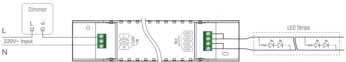
Wiring Diagram
