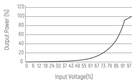
Dimming Curve
