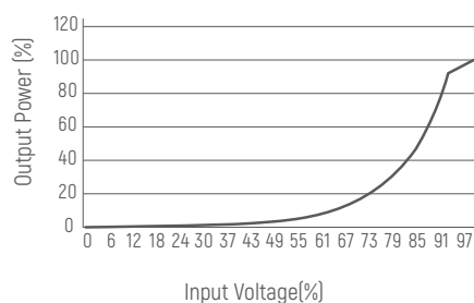
Dimming Curve
