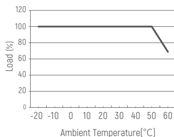
Derating Curve
